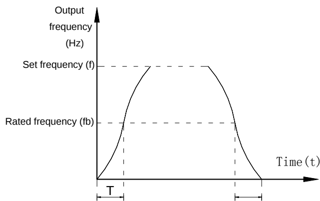
Figure S-curve acceleration/deceleration B
