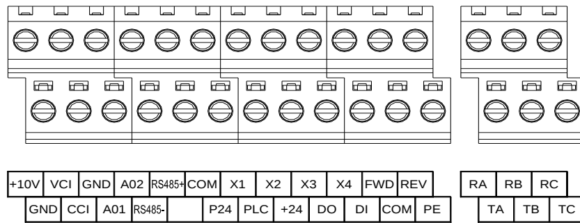
Fig. 3-7 FST-650 series standard control circuit terminal (7.5KW or above)
