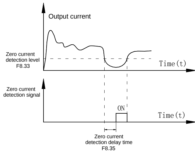
Figure Zero current detectio
