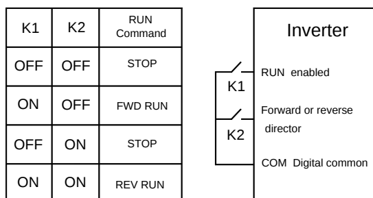
Figure setting of two-line mode 2
