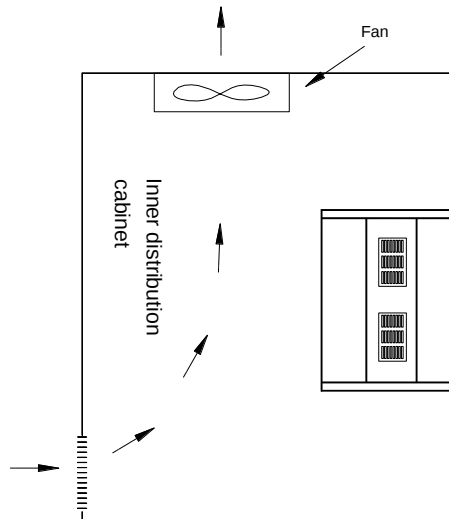
Wrong configuration
