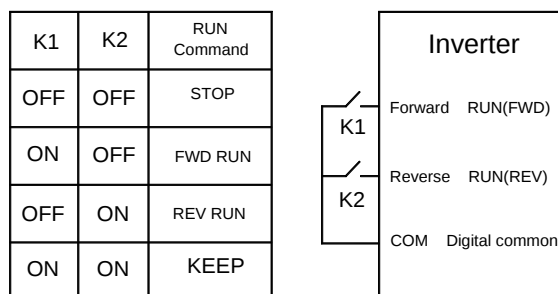
Figure Setting of two-line mode 1
