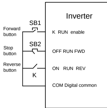
Figure setting of three-line mode 1
