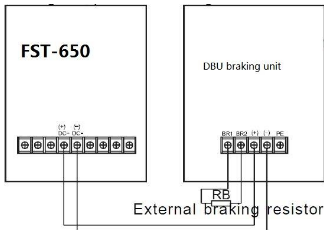
Figure B-1 Connection of Braking resistor
