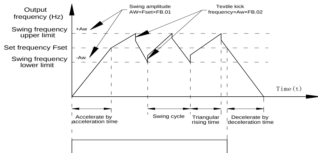
Figure Swing frequency control
