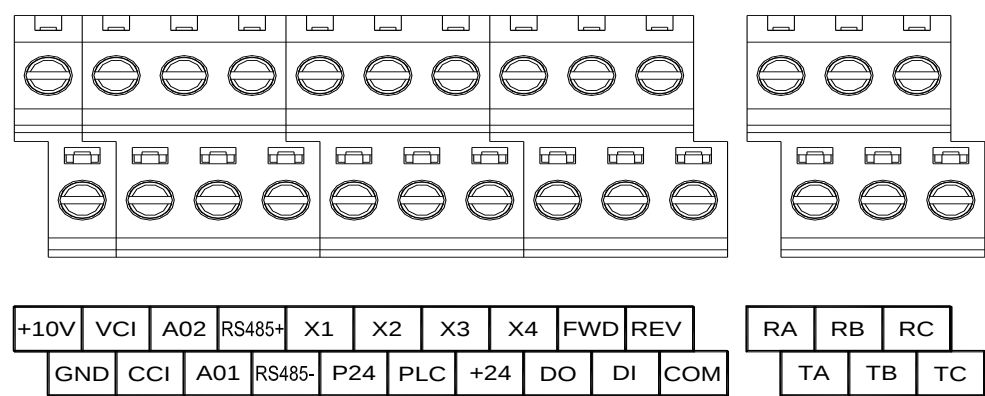
Fig. 3-6 FST-650 series standard control circuit terminal
